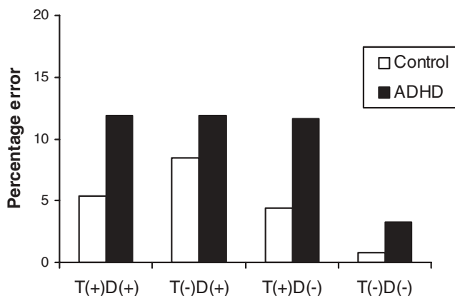
Figure 3 Accuracy (percentage error) for the selective attention task as a function of signal type, plotted for both groups.
